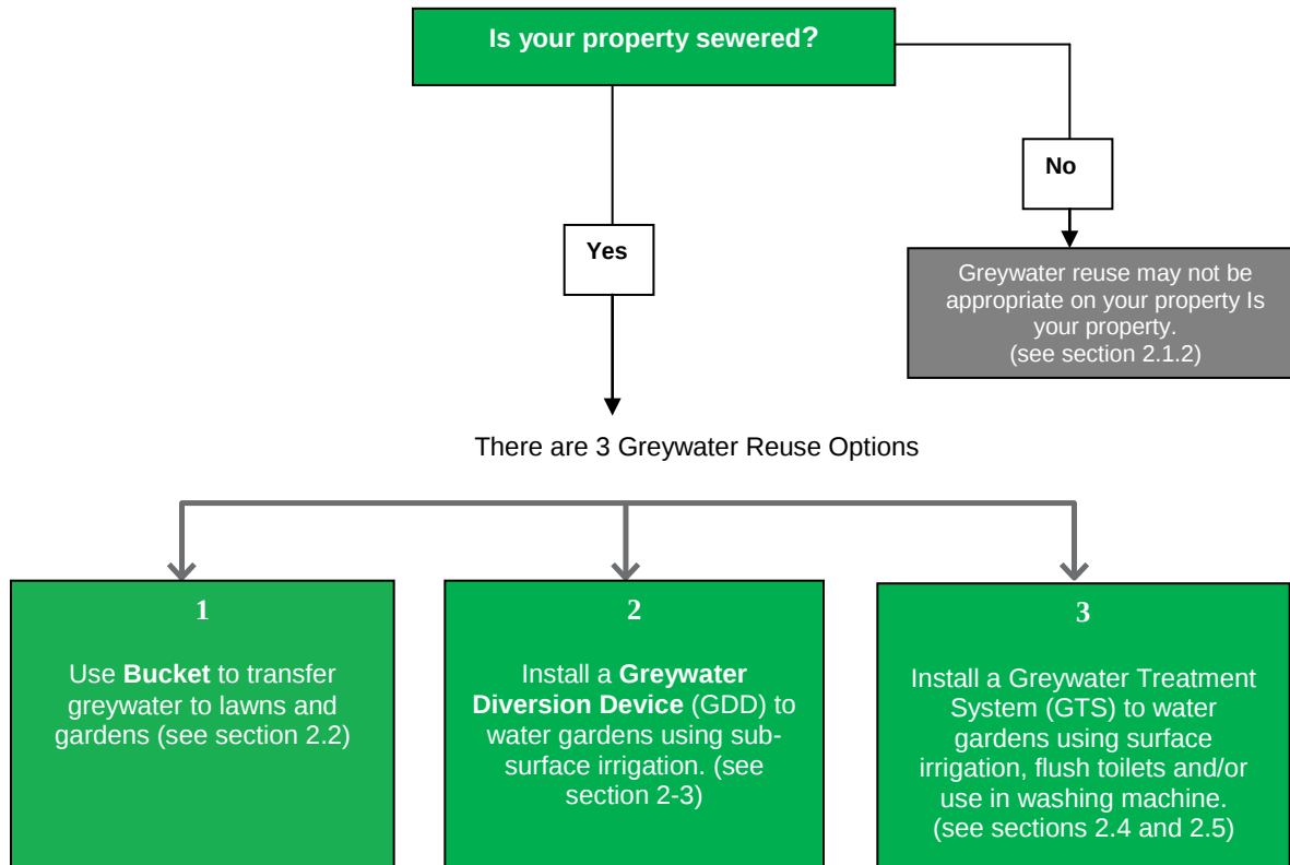
Flowchart 1: Greywater Reuse Option Flowchart for single dwellings
